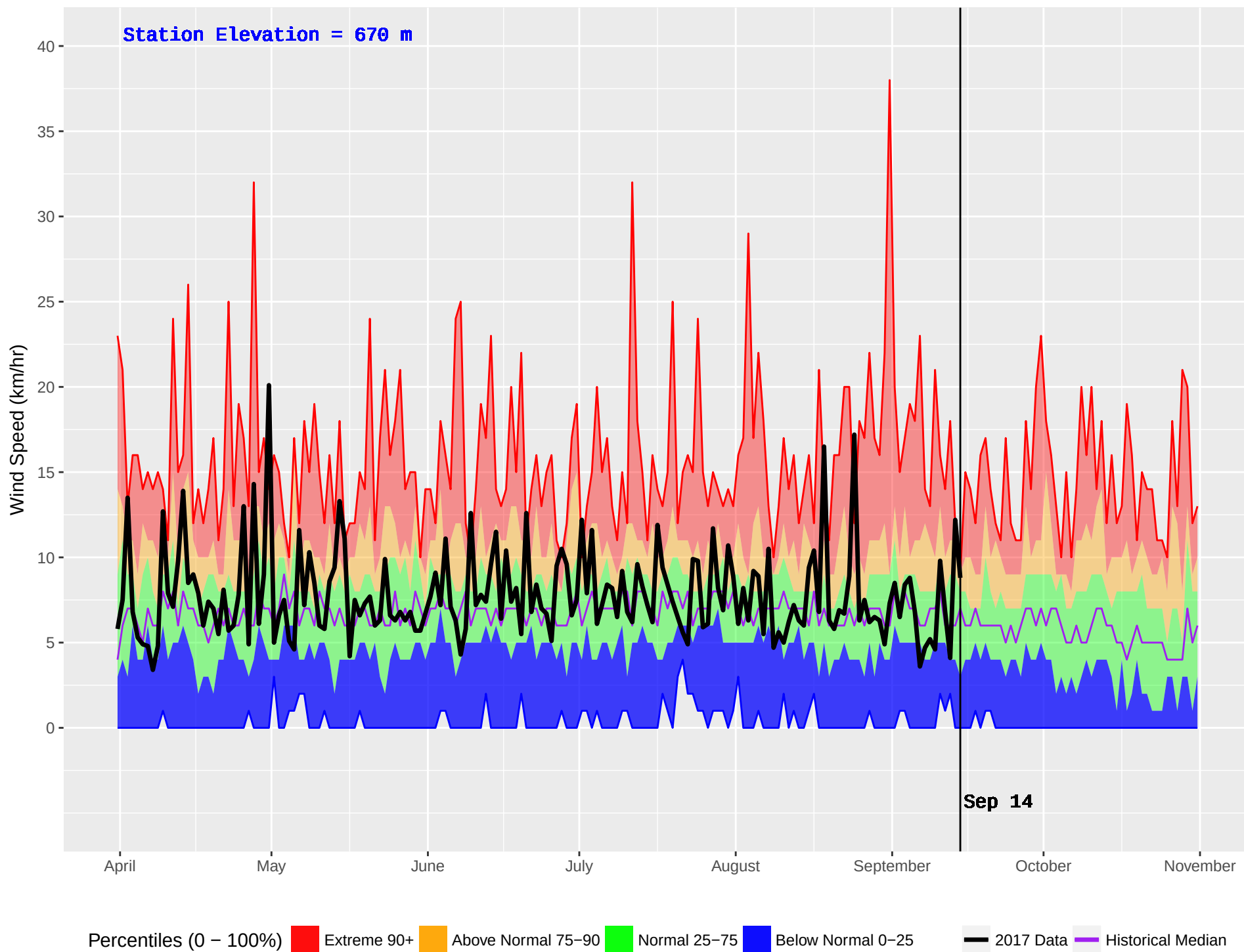
FINTRY (298) : Historical (1989–2016) and Current (2017) Noon Wind Speed
